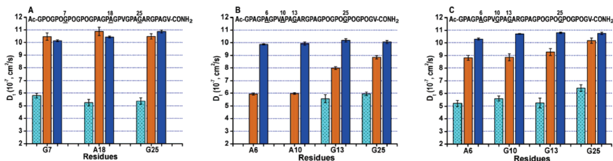
Figure 1. Histogram of the residue-specific diffusion coefficients versus ^{15}\text{N} -labeled residues for (A) T1–892n, (B) T1–892c[G10A], and (C) T1–892c. D_{\text{T}}^{10^\circ\text{C}} , D_{\text{M}}^{10^\circ\text{C}} , and D_{\text{M}}^{40^\circ\text{C}} are shown in dotted cyan, orange, and blue, respectively.
